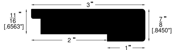
Square Stair Nose (782)
