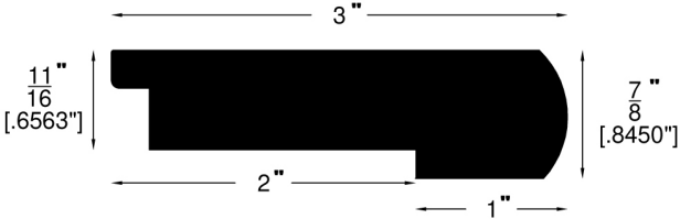
Stair Nose (781)
