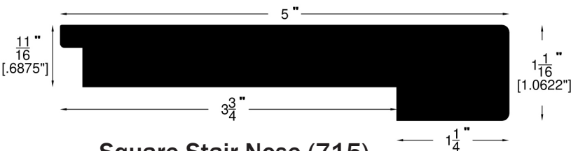
Square Stair Nose (715)
