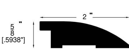
Reducer (780)
