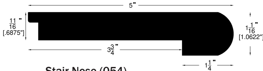
Stair Nose (054)
