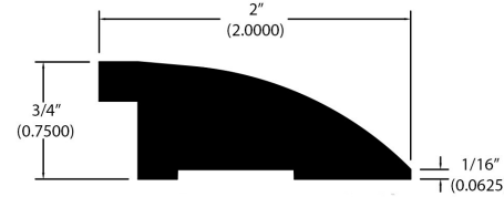
Reducer (716)
