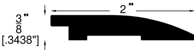
Reducer (707)
