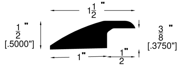
Reducer Overlap (747)
