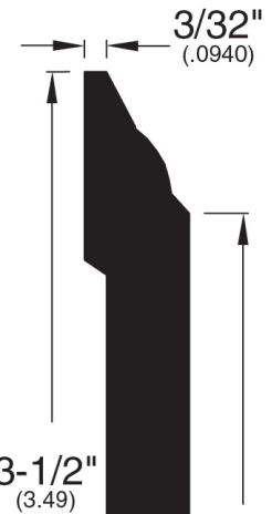
Reducer Overlap (747)
