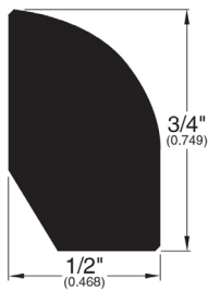
Base Shoe (024)
