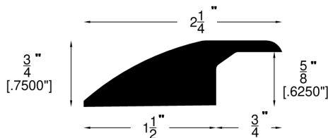
Reducer Overlap (749)
