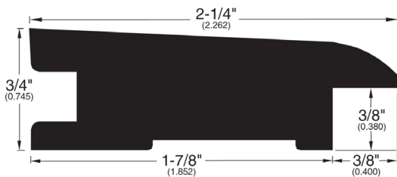
Reducer (045)
