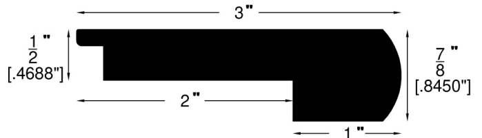
Stair Nose (712)
