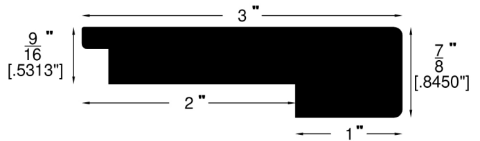
Stair Nose (719)
