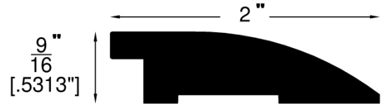
Reducer (720)
