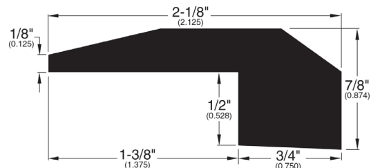
Threshold (011)
