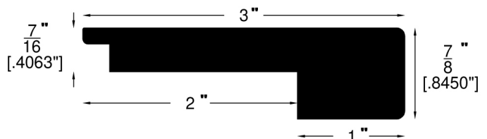
Stair Nose (743)
