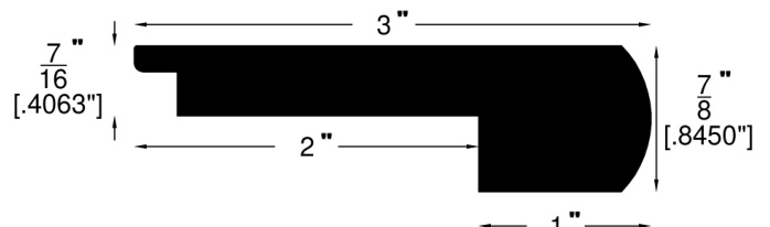
Stair Nose (742)
