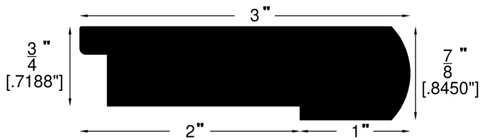
Stair Nose (717)
