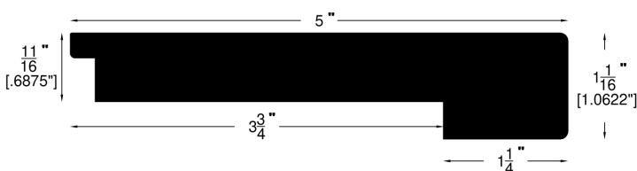
Stair Nose (715)
