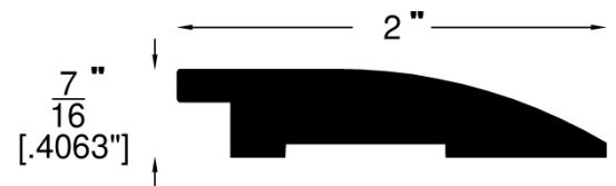
Reducer (741)
