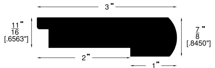
Stair Nose (781)
