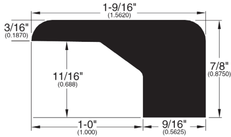
Square Nose (027)
