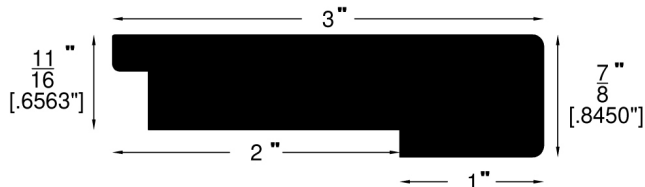
Stair Nose (782)
