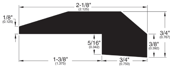
Threshold (008)
