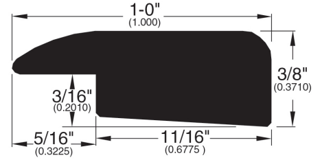
Square Nose (243)
