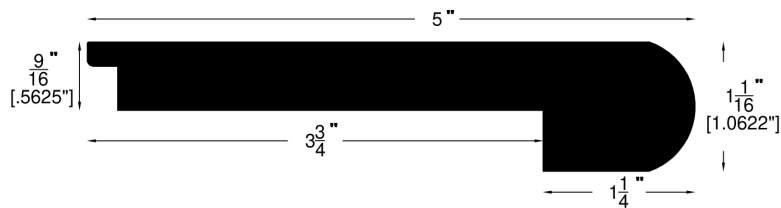
Stair Nose (154)
