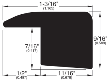
Square Nose (043)
