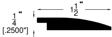
Reducer (722)
