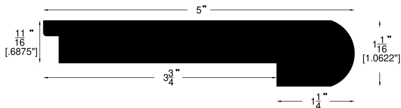
Stair Nose (054)
