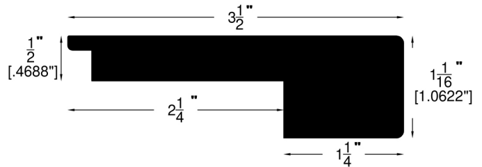
Stair Nose (714)
