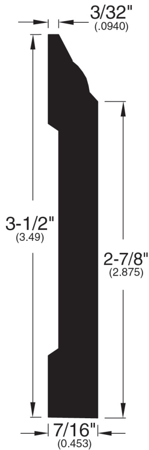
Wall Base (003)
