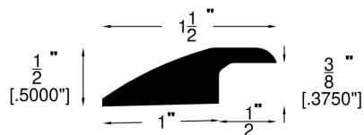
Reducer Overlap (747)
