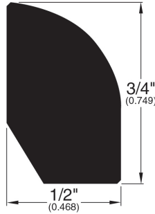
Base Shoe (024)
