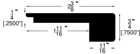
Stair Nose (724)
