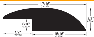
Reducer Overlap (329)
