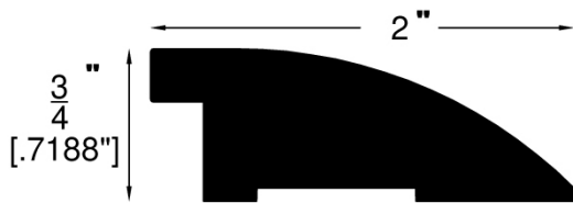
Reducer (716)
