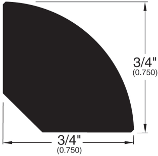
Quarter Round (001)
