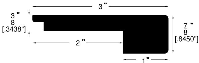
Stair Nose (708)
