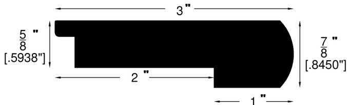
Stair Nose (738)
