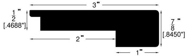
Stair Nose (713)
