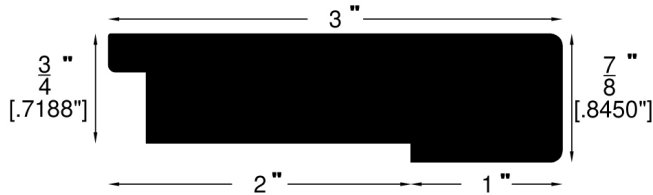
Stair Nose (718)
