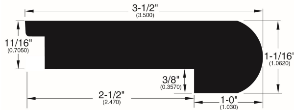
Stair Nose (761)
