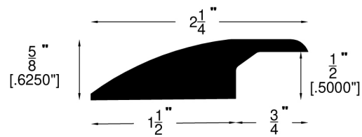
Reducer Overlap (748)
