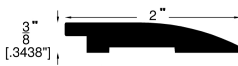
Reducer (707)
