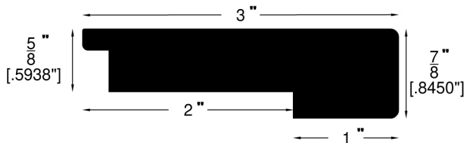
Stair Nose (739)
