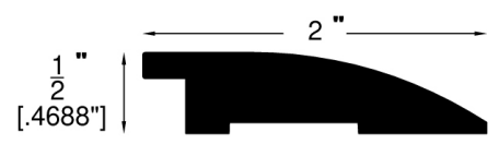
Reducer (710)
