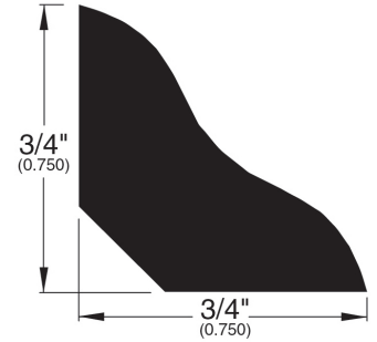
Cove (073)
