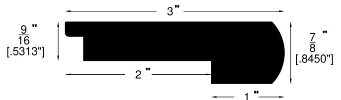
Stair Nose (721)
