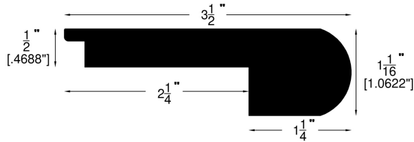
Stair Nose (750)
