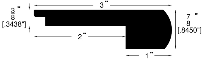
Stair Nose (709)
