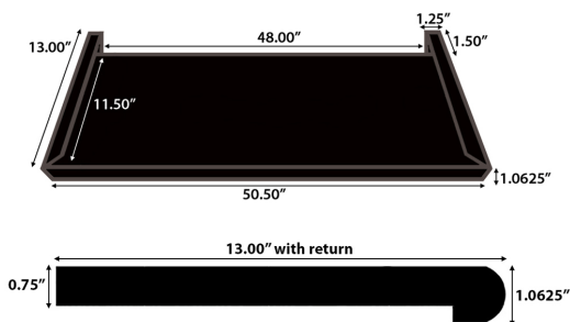
36", 42", 48" Round Nose Universal Tread
