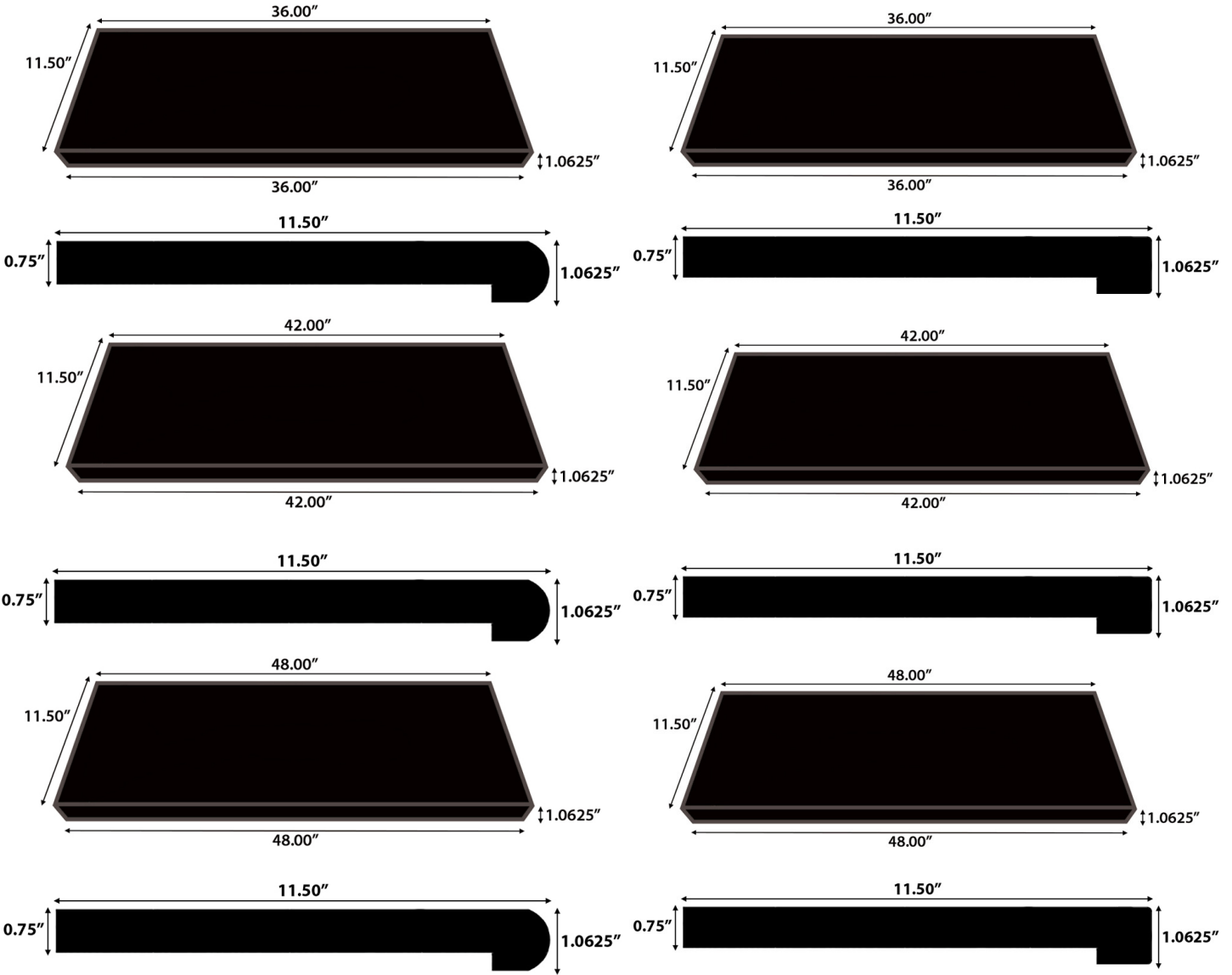
36", 42", 48" Round Nose Standard Tread
