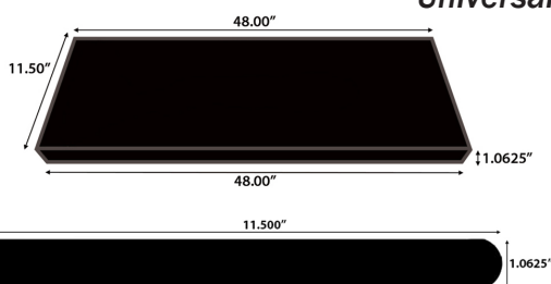
36", 42", 48" Round Nose Full Thickness Tread
