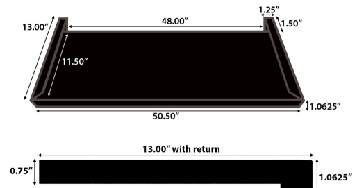
36", 42", 48" Square Nose Universal Tread
