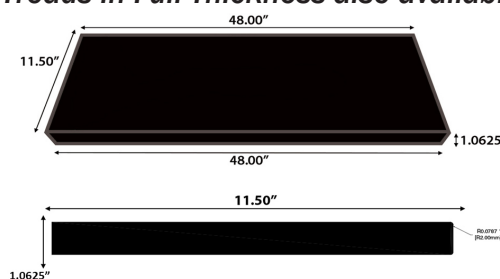
36", 42", 48" Square Nose Full Thickness Tread
